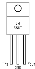
TO-220 Plastic Package*
