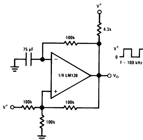
Squarewave Oscillator
