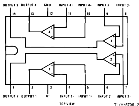
Dual-In-Line Package
