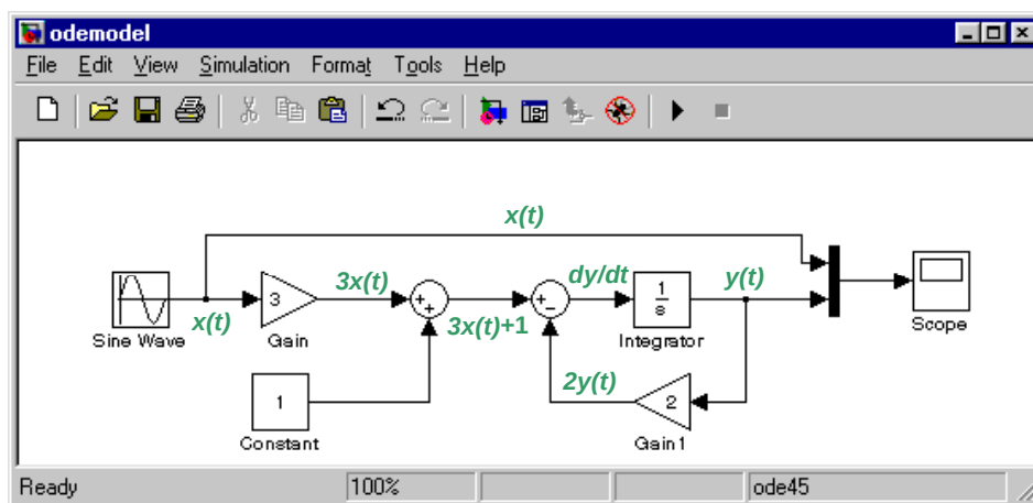
Figure 10 Simulink model of a linear, first-order ODE
