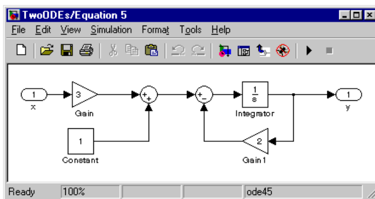
Figure 13 Equation 5 subsystem
