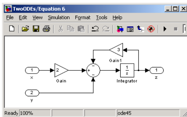
Figure 14 Equation 6 subsystem
