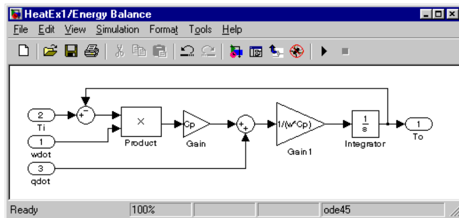
Figure 19 Energy balance subsystem
