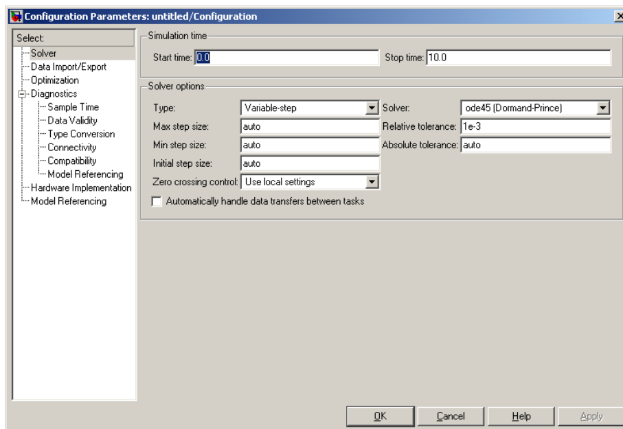
Figure 7 Simulation parameters menu, Solver panel
