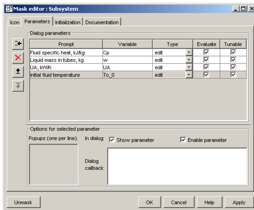
Figure 24 Mask editor with block parameters defined
