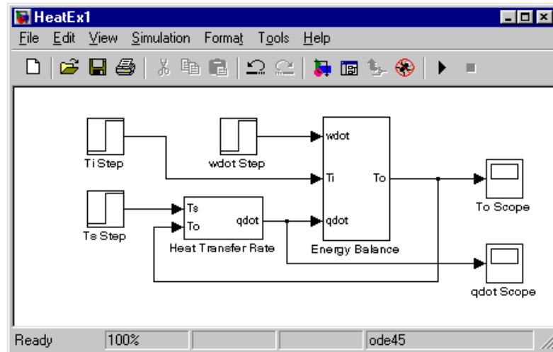
Figure 17 Heat exchanger model -- main window
